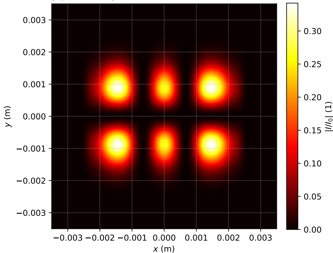
Intensity profile I(x, y, z = 3.105)/I_0 , P_{in}=1.0P_{cr} , artificial time
